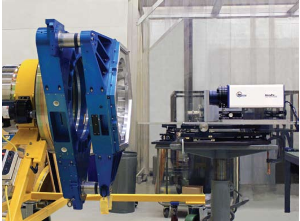
Figure 3. Vibration-Insensitive AccFiz Interferometer at NOAO's Optics Shop facility, shown here measuring components for the WIYN telescope's One Degree Imager.
